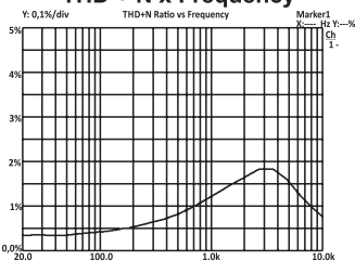
THD + N x Frequency
