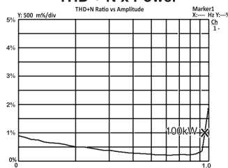
THD + N x Power
