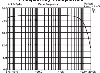
Frequency Response
