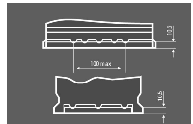
Base holddown
