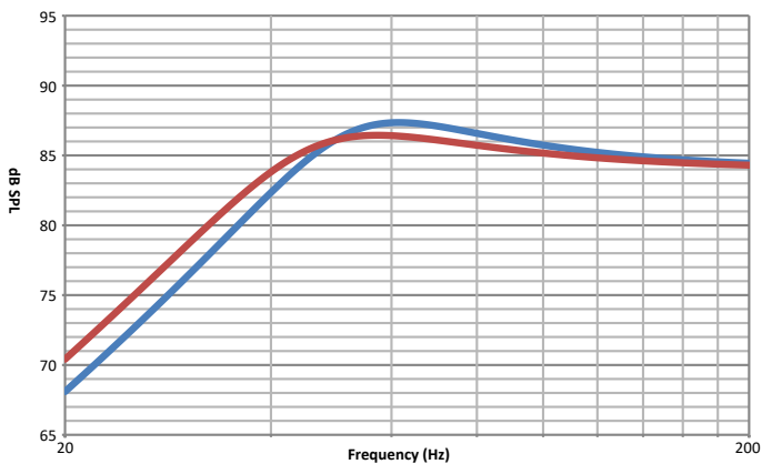
P25FS Closed box frequency response
