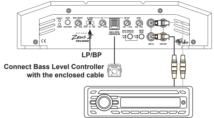
Connect stereo RCA output (L/R or SUB OUT) of the head unit with LINE IN of the amplifier
