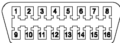
Pin allocation OBD, front view
