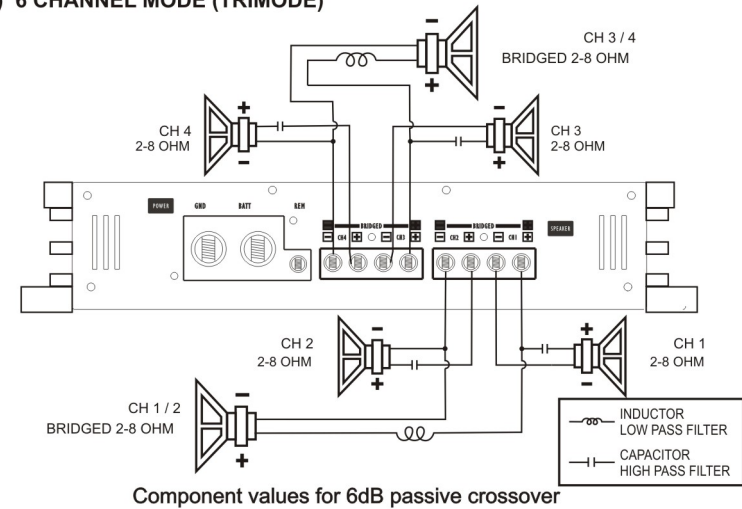
Component values for 6dB passive crossover
