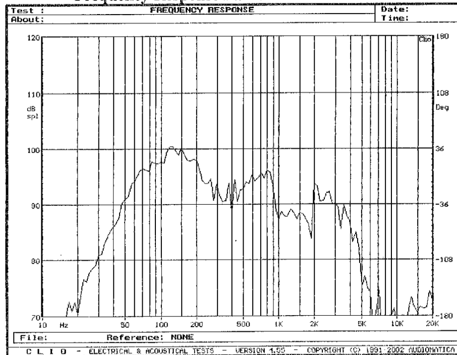
Frequency Response Baffle IEC – 2.83 V – 1m
