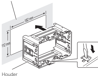
Dashboard
