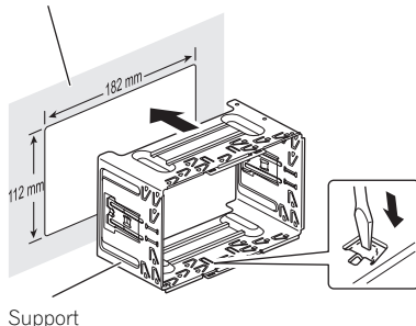
Support
