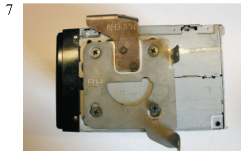
Mount the original bracket on the new headunit.
