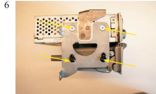
Remove the original mounting bracket. This is tighten by eight screws.
