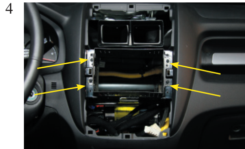
Place the metal bracket. Tighten the bracket by four Philips screws. Place the headunit.
