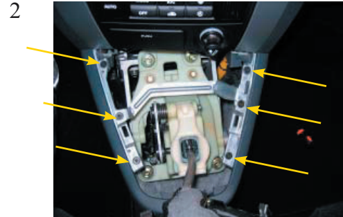
Remove the screws at the location of the arrows. Remove the metal ring.
