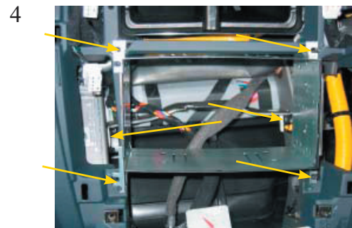
Place the metal bracket and tighten the four screws. Remove the original bracket which is indicated at the middle arrows
